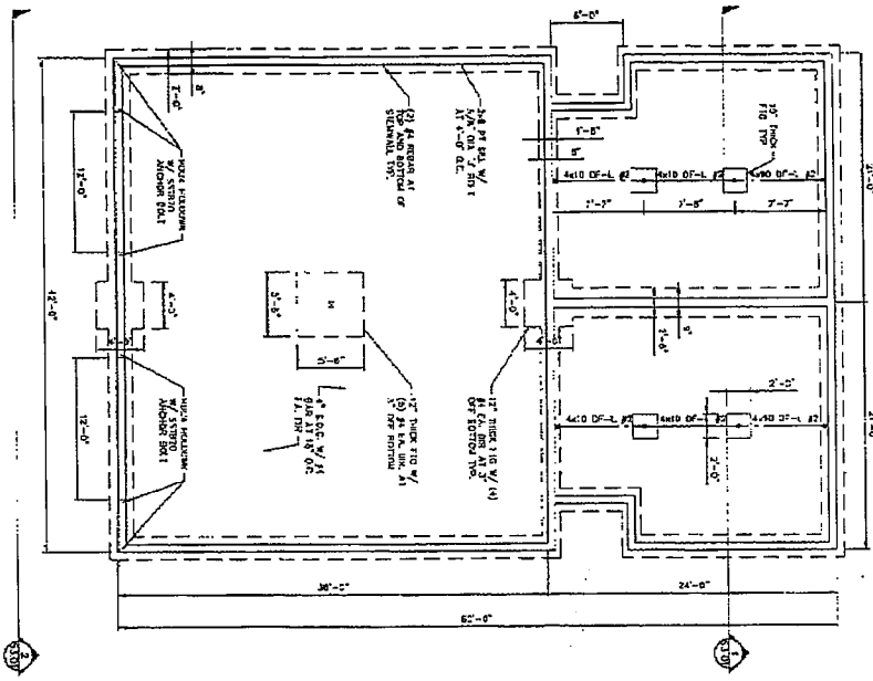
1 FOUNDATION PLAN S1.01 3/18-1'-0"
