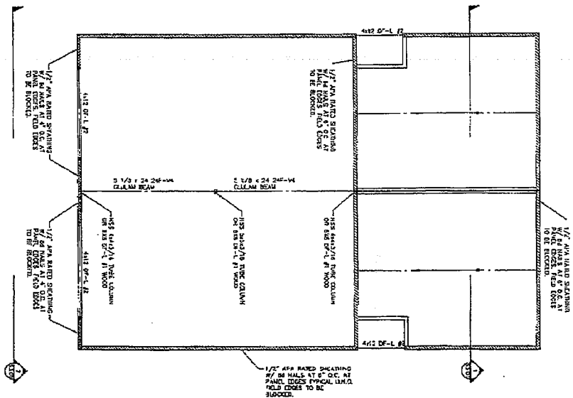
2 MAIN FLOOR PLAN S1.01 3/18-1'-0"
